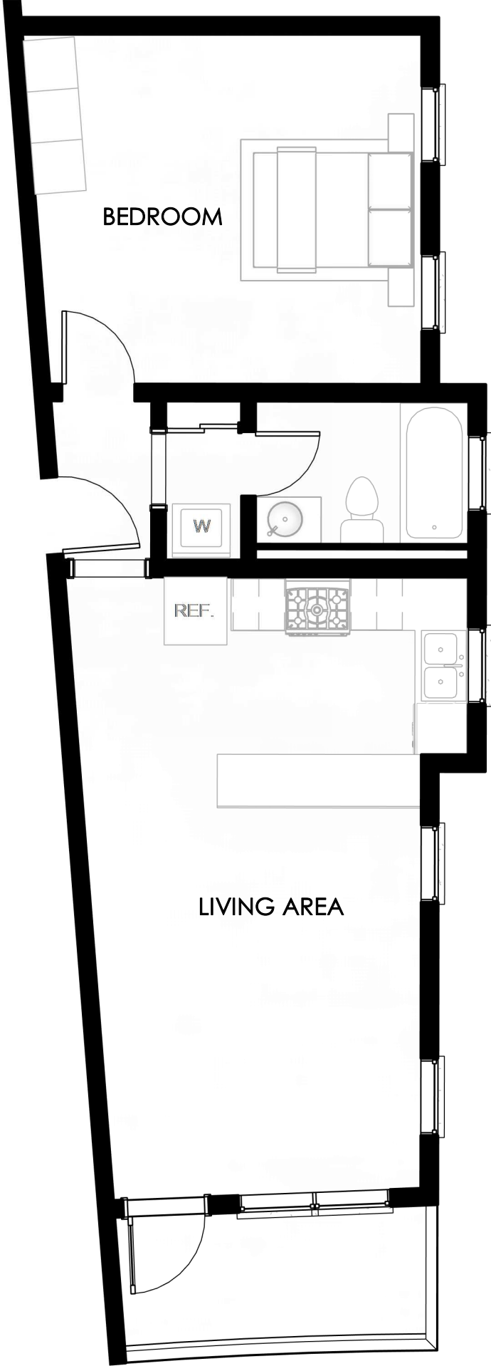
2 BLDG B_UNIT 4 - 1 BEDROOM AREA: 736 SF 3/16" = 1'-0"
