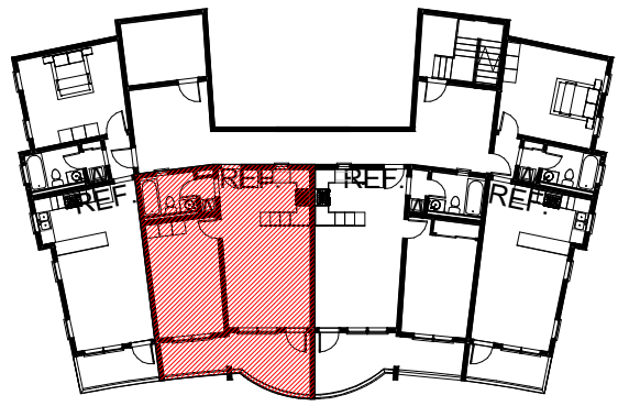
1 BB_LEVEL 1-3 1/32" = 1'-0"
