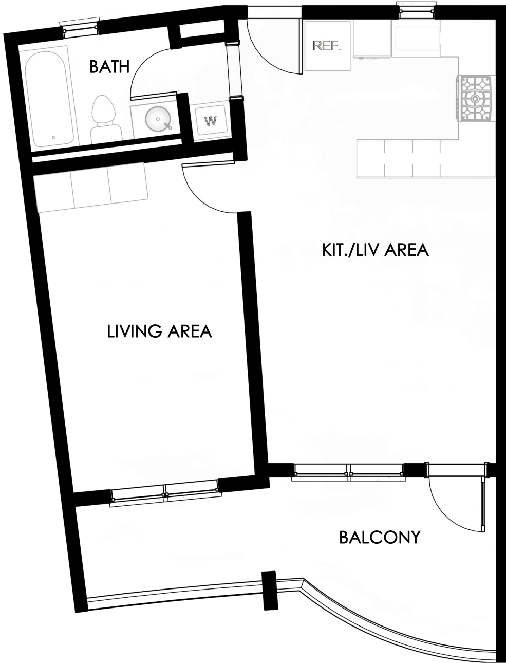
2 BLDG B/C_UNIT 2 - 1 BEDROOM 3/16" = 1'-0" AREA: 771 SF
